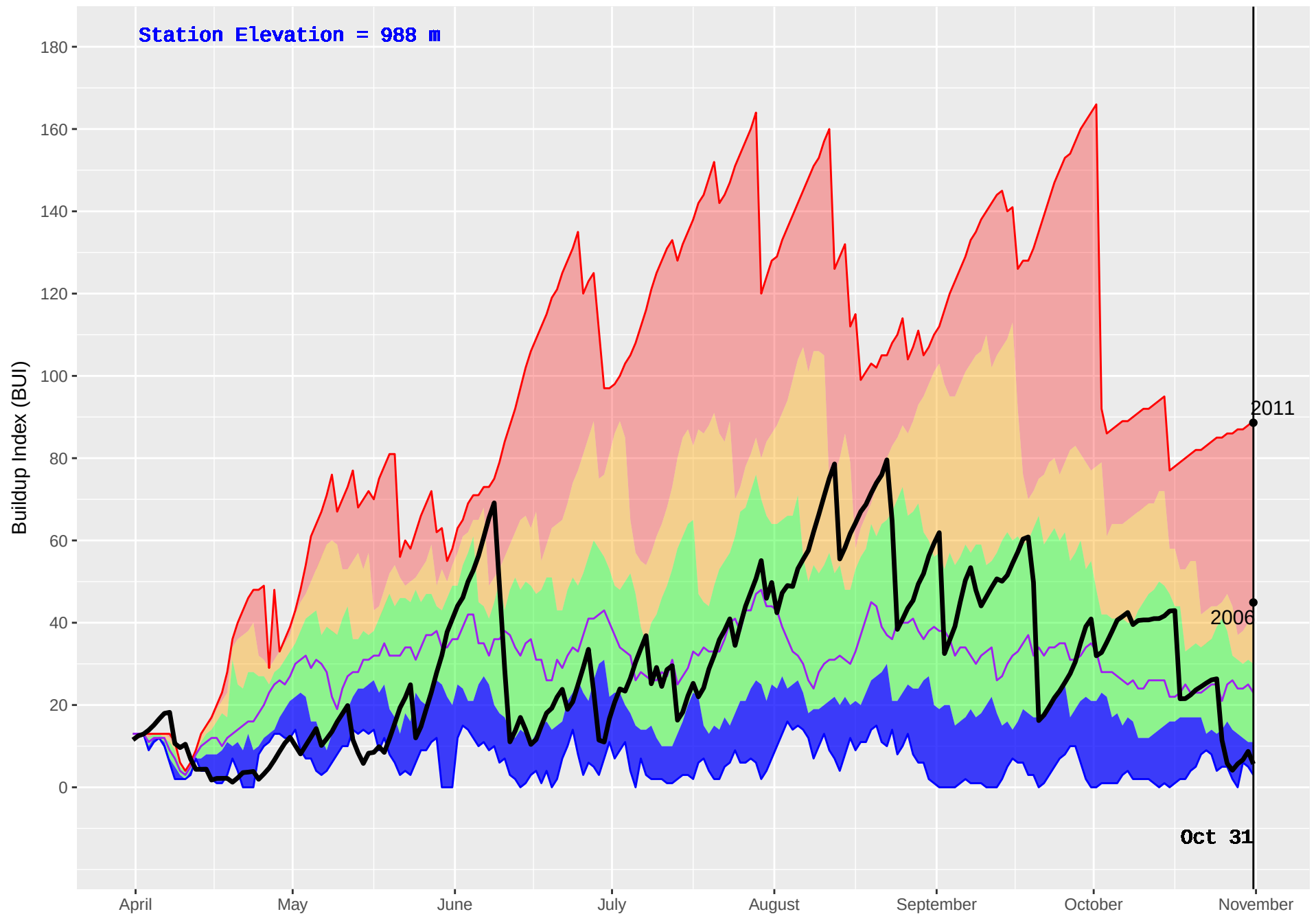
NOEL (437) : Historical (1993–2016) and Current (2017) Noon Buildup Index (BUI)
