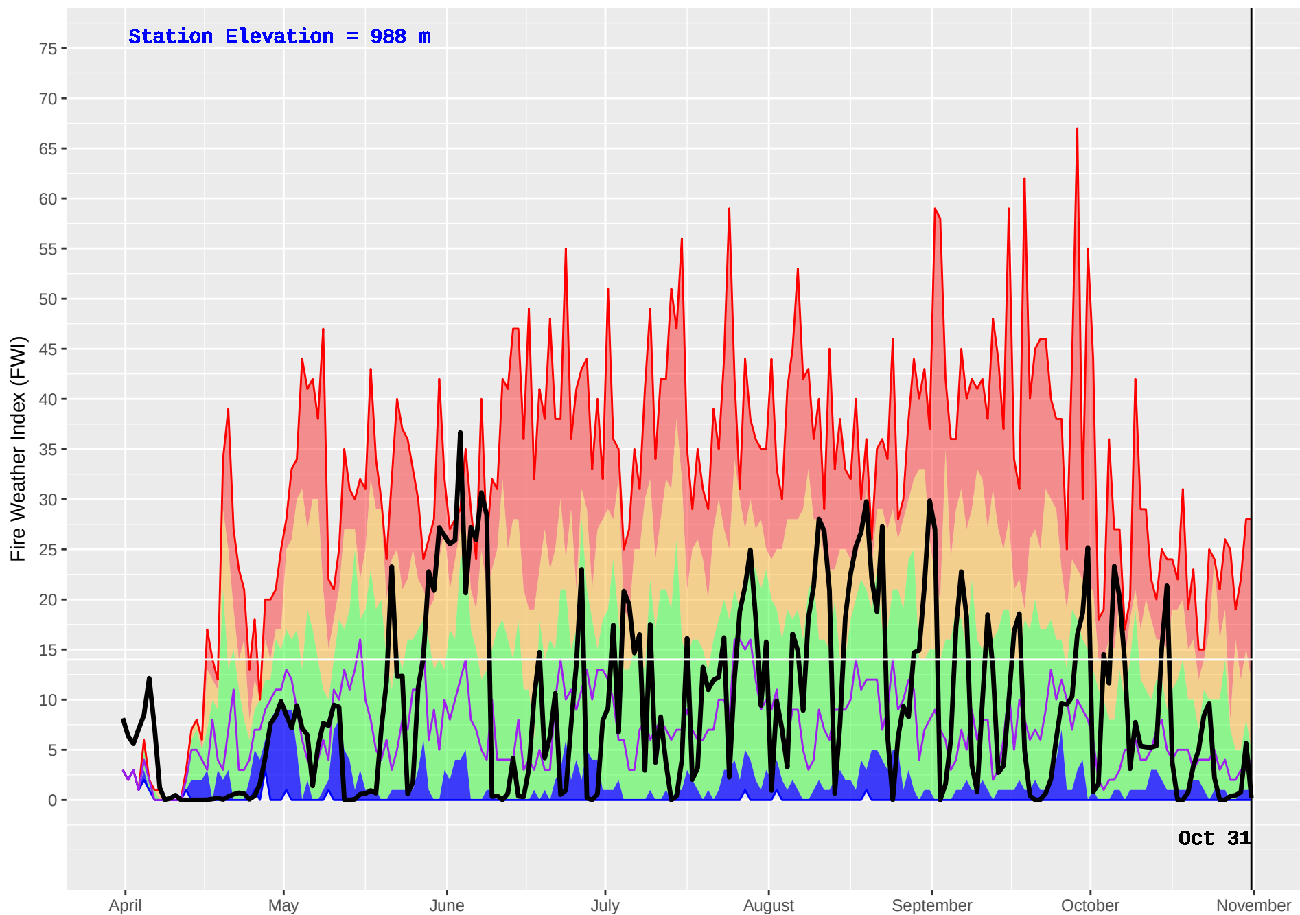
NOEL (437) : Historical (1993–2016) and Current (2017) Noon Fire Weather Index (FWI)
