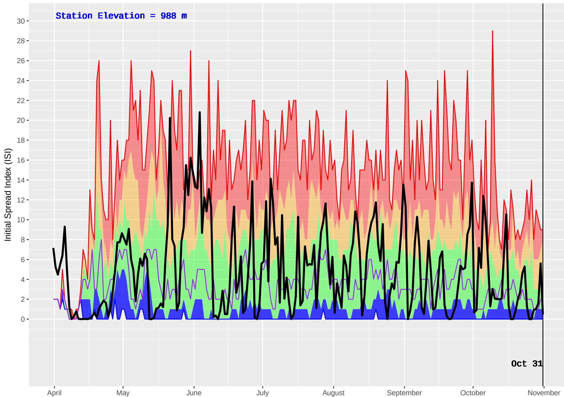
NOEL (437) : Historical (1993–2016) and Current (2017) Noon Initial Spread Index (ISI)
