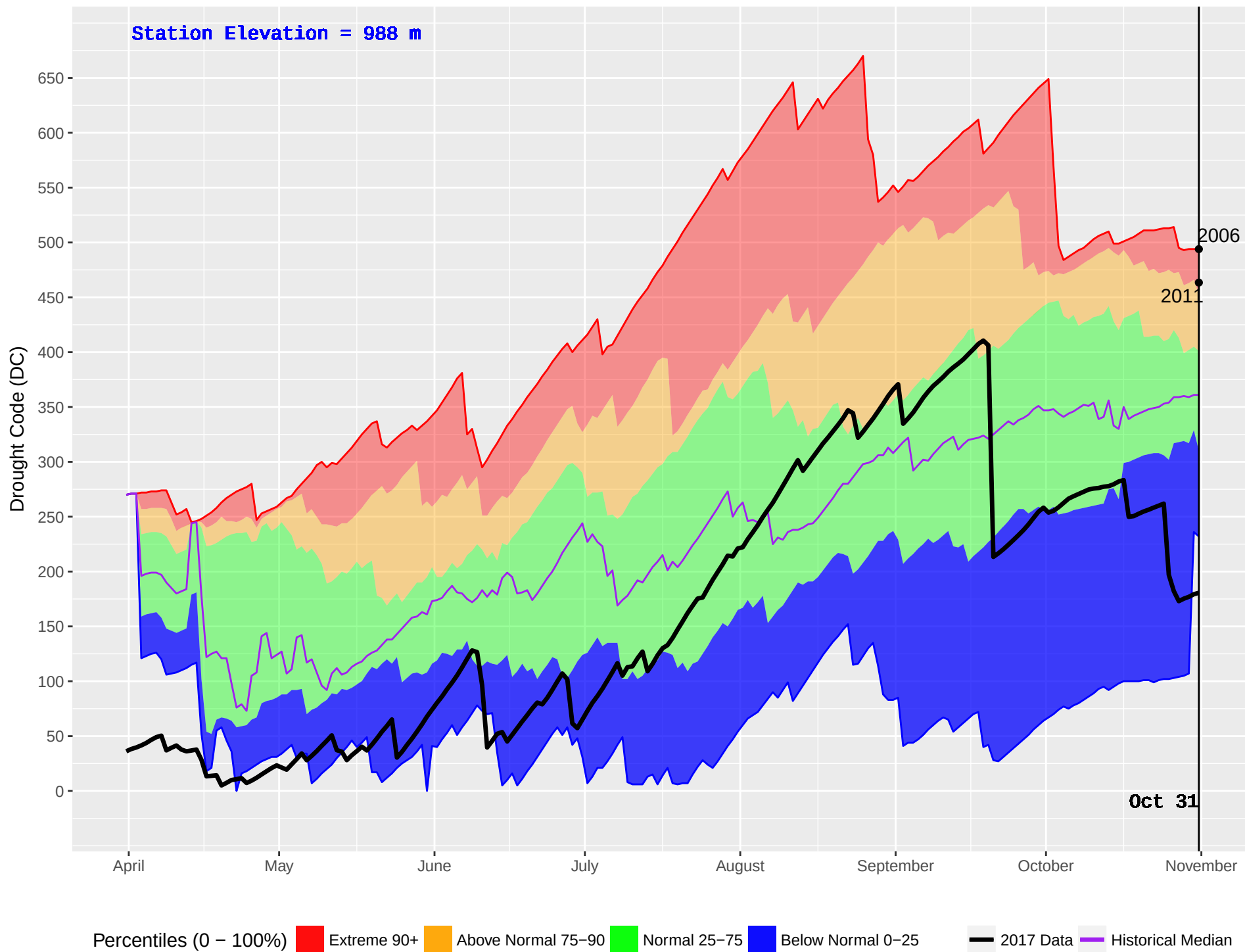
NOEL (437) : Historical (1993–2016) and Current (2017) Noon Drought Code (DC)
