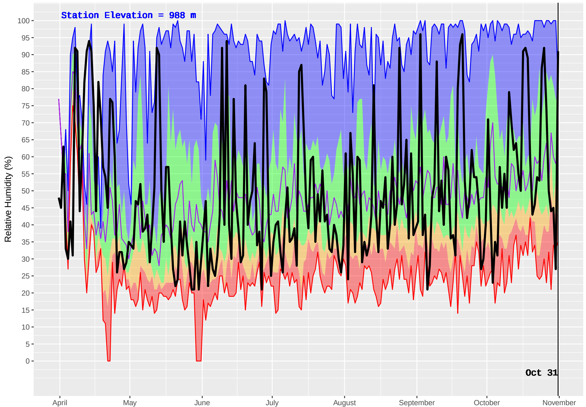
NOEL (437) : Historical (1993–2016) and Current (2017) Noon Relative Humidity
