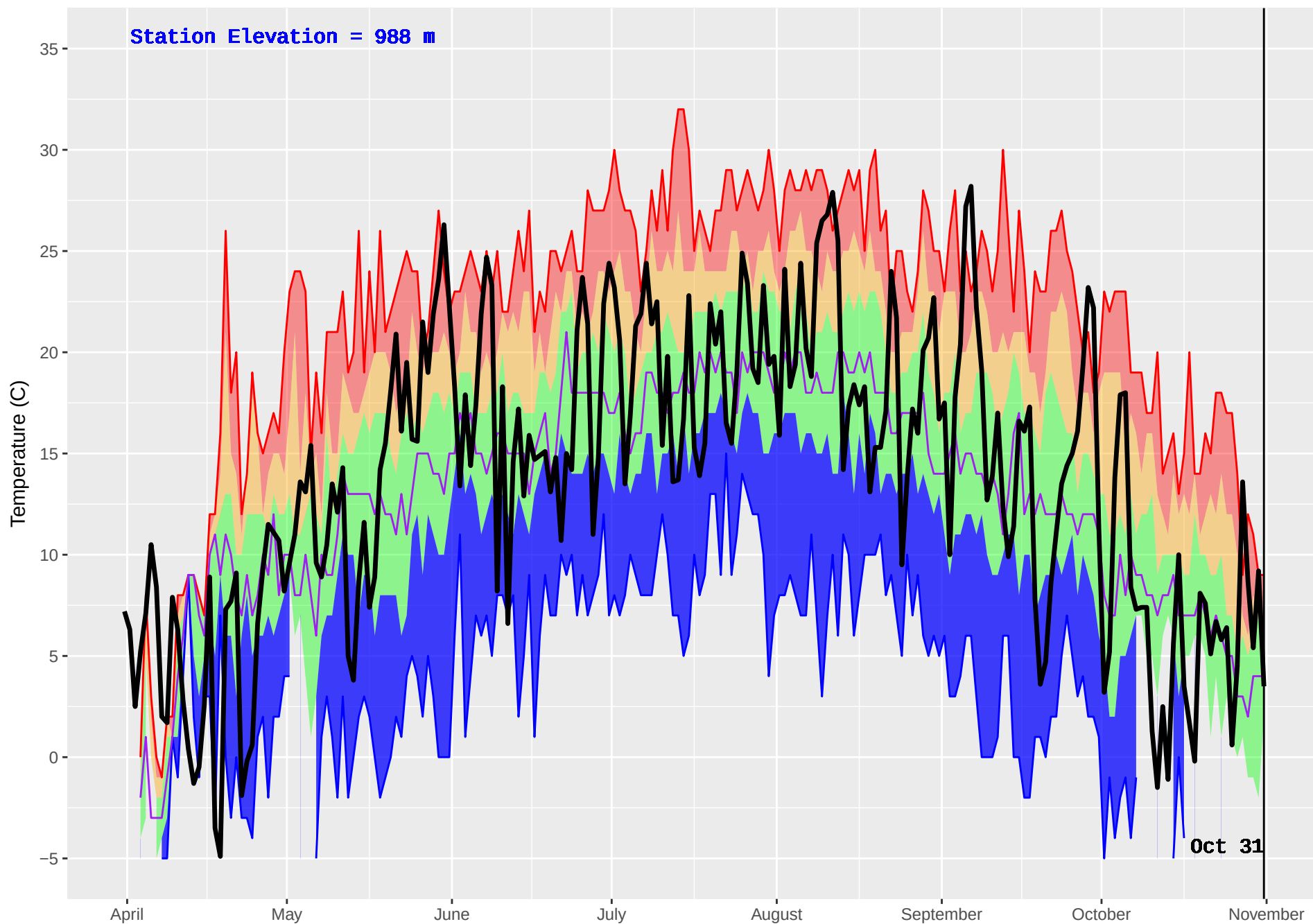
NOEL (437) : Historical (1993–2016) and Current (2017) Noon Temperature
